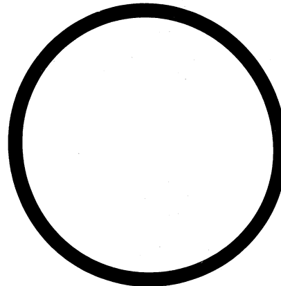
PN 00-3084-56 1.937 I.D. X 2.125 O.D. x 0.094 QUAD-RING/BUNA-N
