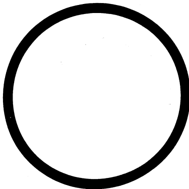
PN 00-3084-11 1.750 I.D. X 1.937 O.D. x 0.093 TETRASEAL/BUNA-N
